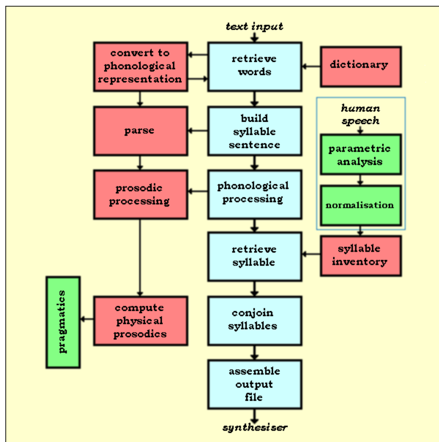
Fig. 1 SPRUCE text-to-speech synthesis.
